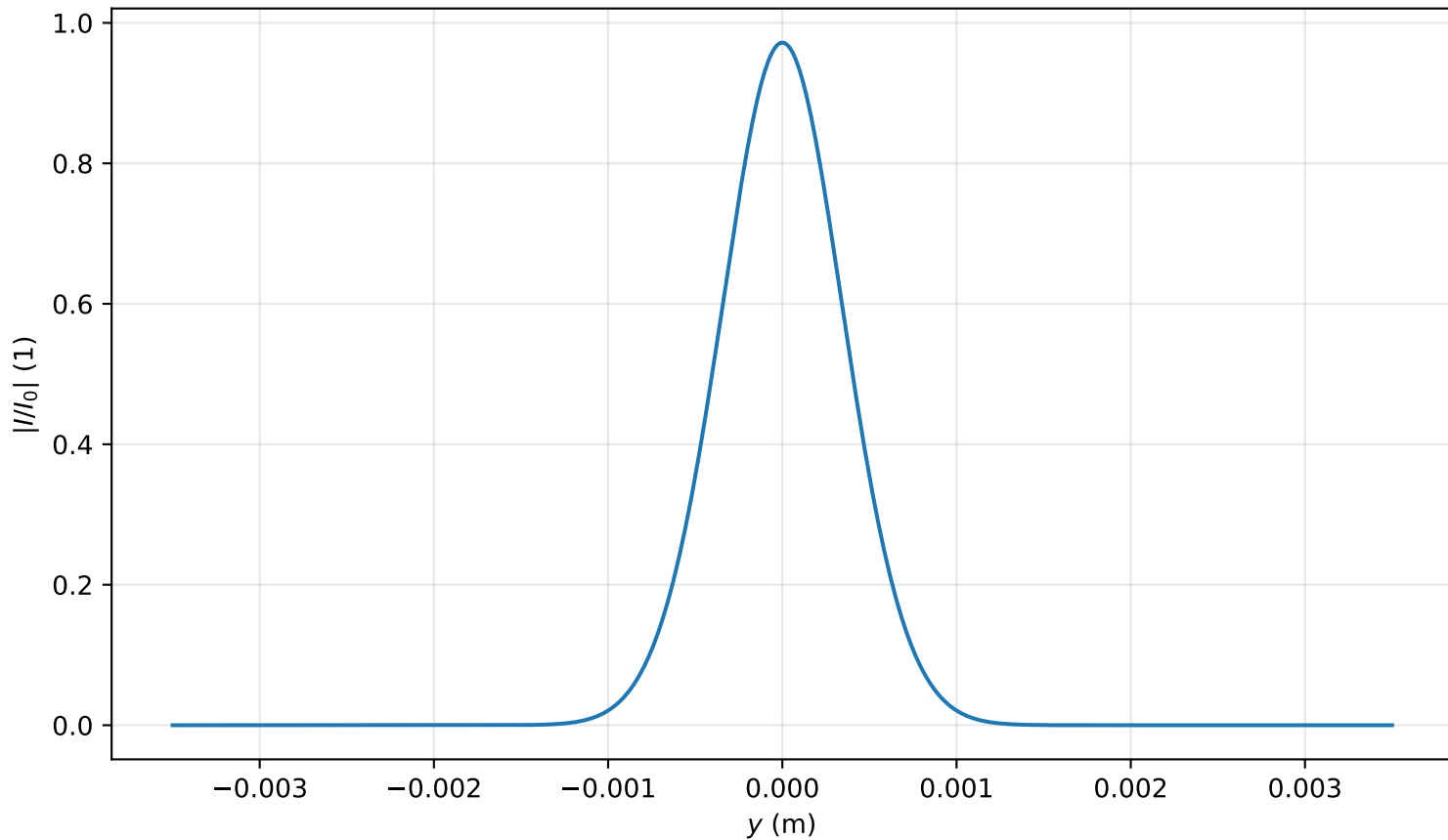
Intensity profile I(x=0, y, z=0.557)/I_0 , P_{in}=0.2P_{cr} , artificial time
